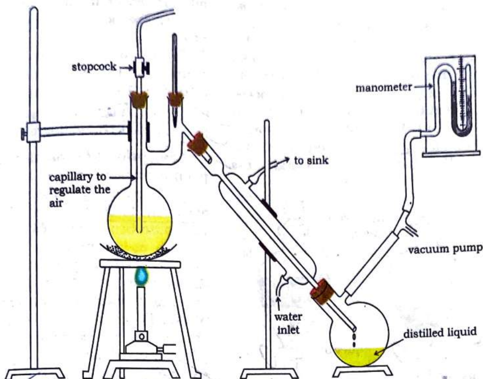
Fig.12.8 Distillation under reduced pressure. A liquid boils at a temperature below its vapour pressure by reducing the pressure.
