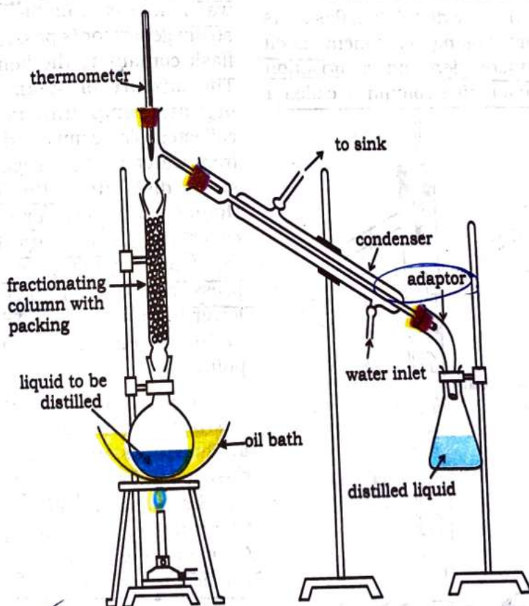
Fig. 12.6 Fractional distillation. The vapours of lower boiling fraction reach the top of the column first followed by vapours of higher boiling fractions.
