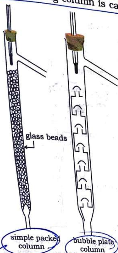
Fig. 12.7 Different types of fractionating columns.
