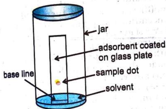
Fig. 12.12 (a) Thin layer chromatography. Chromatogram being developed.
