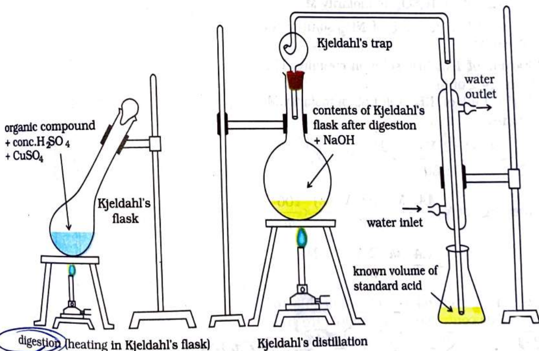
Fig. 12.16 Kjeldahl method. Nitrogen-containing compound is treated with concentrated H_2SO_4 to get ammonium sulphate which liberates ammonia on treating with NaOH; ammonia is absorbed in known volume of standard acid.
