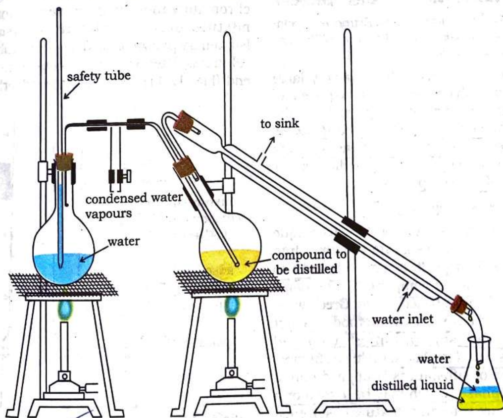
Fig.12.9 Steam distillation. Steam volatile component volatilizes, the vapours condense in the condenser and the liquid collects in conical flask.
