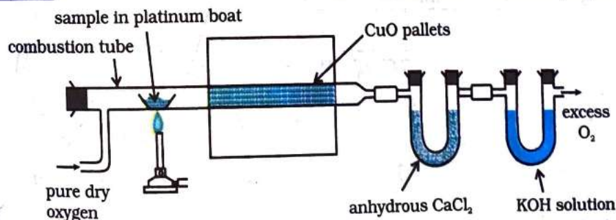
Fig.12.14 Estimation of carbon and hydrogen. Water and carbon dioxide formed on oxidation of substance are absorbed in anhydrous calcium chloride and potassium hydroxide solutions respectively contained in U tubes.
