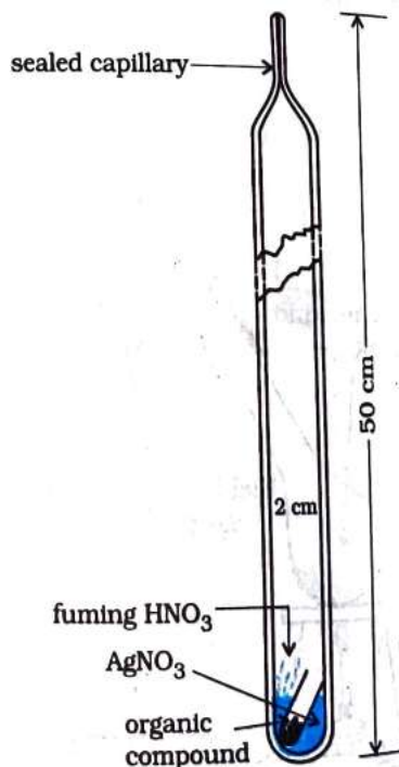
Fig. 12.17 Carius method. Halogen containing organic compound is heated with fuming nitric acid in the presence of silver nitrate.
