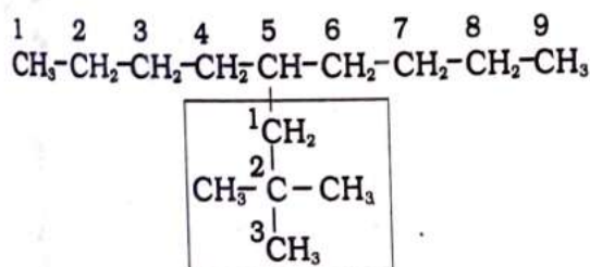
5-(2,2-Dimethylpropyl)nonane
