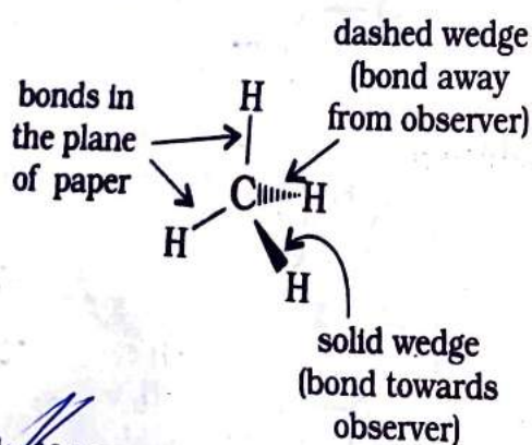
Fig. 12.1 Wedge-and-dash representation of \text{CH}_4
