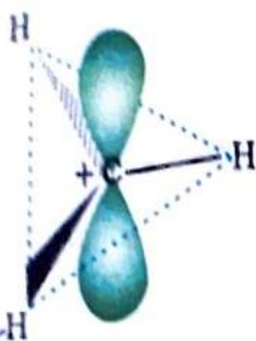
Fig. 12.3 Shape of methyl cation
