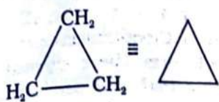
Cyclopropane
