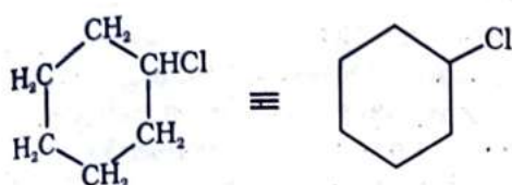
chlorocyclohexane
