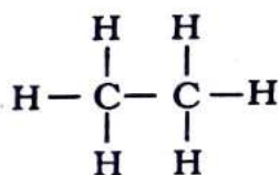
Ethane
