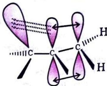
Fig. 12.4(b) Orbital diagram showing hyperconjugation in propene
