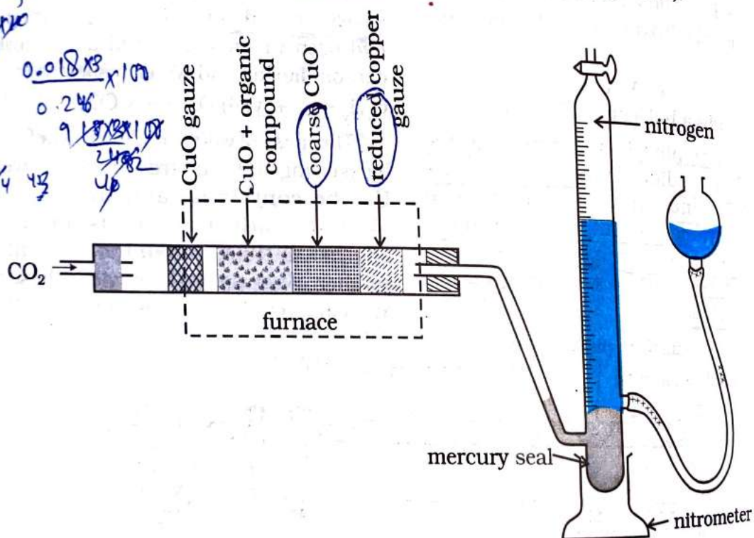
Fig. 12.15 Dumas method. The organic compound yields nitrogen gas on heating it with copper(II) oxide in the presence of CO_2 gas. The mixture of gases is collected over potassium hydroxide solution in which CO_2 is absorbed and volume of nitrogen gas is determined.
