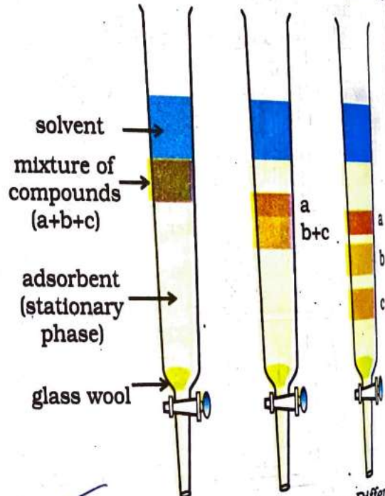
Fig.12.11 Column chromatography. Different stages of separation of components of a mixture.
