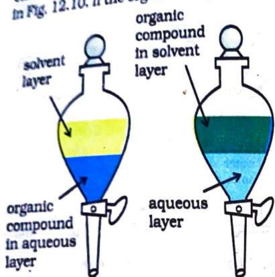
Fig.12.10 Differential extraction. Extraction of compound takes place based on difference in solubility
