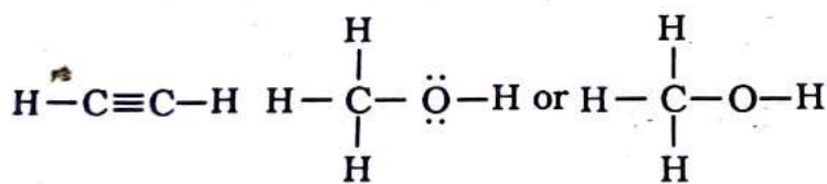
Ethyne
