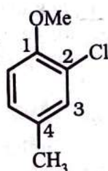
2-Chloro-4-methylanisole
