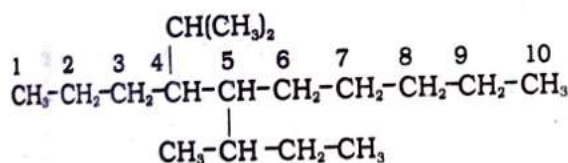
5-sec-Butyl-4-isopropyldecane
