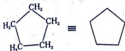
Cyclopentane
