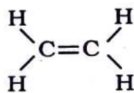
Ethene
